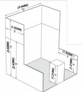
PERIMETER BOOTH 3D VIEW
